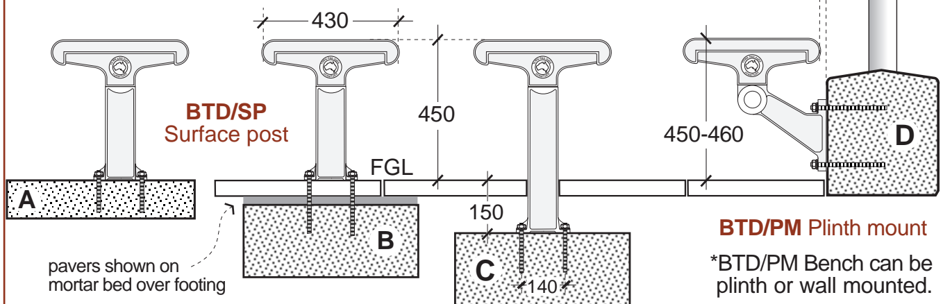
BTD/SS Sub-surface post
